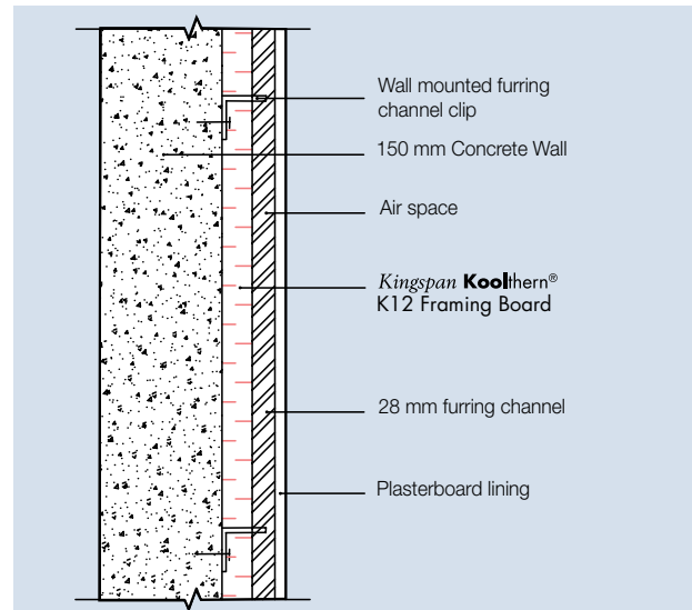
Figure 6 Side elevation of Kingspan Kooltherm ® K12 Framing Board clip-and-channel system
